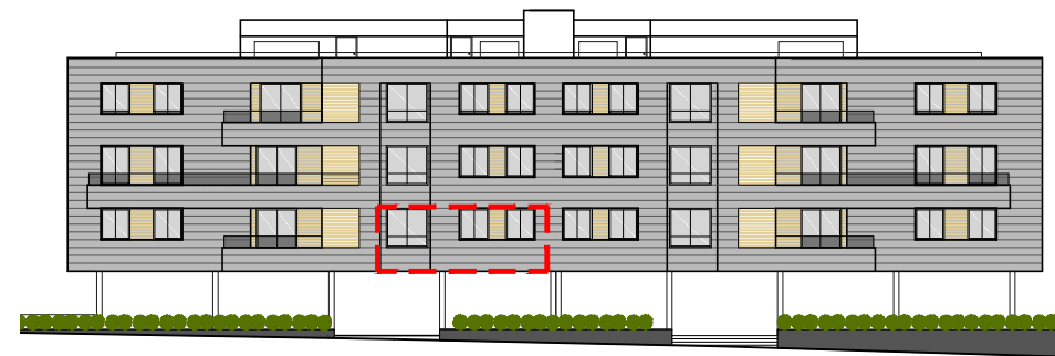
ALZADO PRINCIPAL
